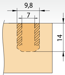
FIYU® FAST and FIYU® LOCK
