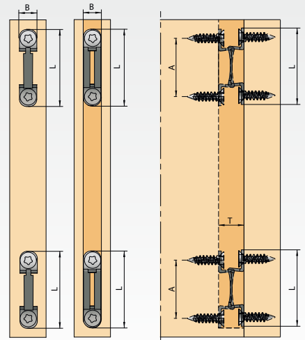
Assembling cabinet body with MODULAR
